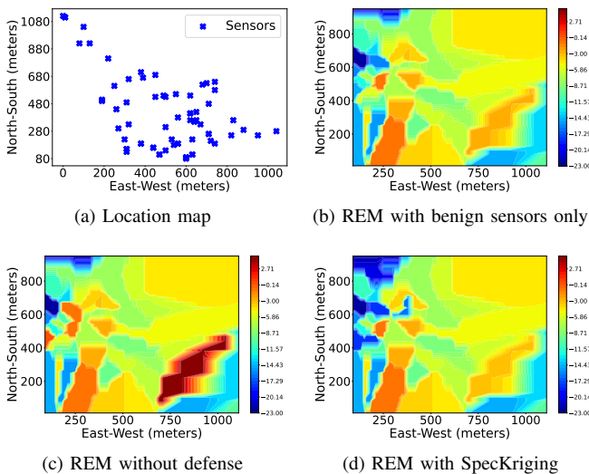
Fig. 9: REMs of heterogeneous nodes.
