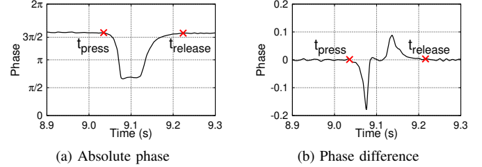
Fig. 5. Absolute and differential phase changes caused by a single tap.
