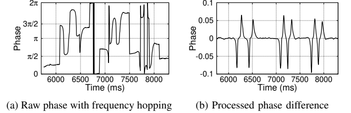
Fig. 6. Data processing under frequency hopping.
