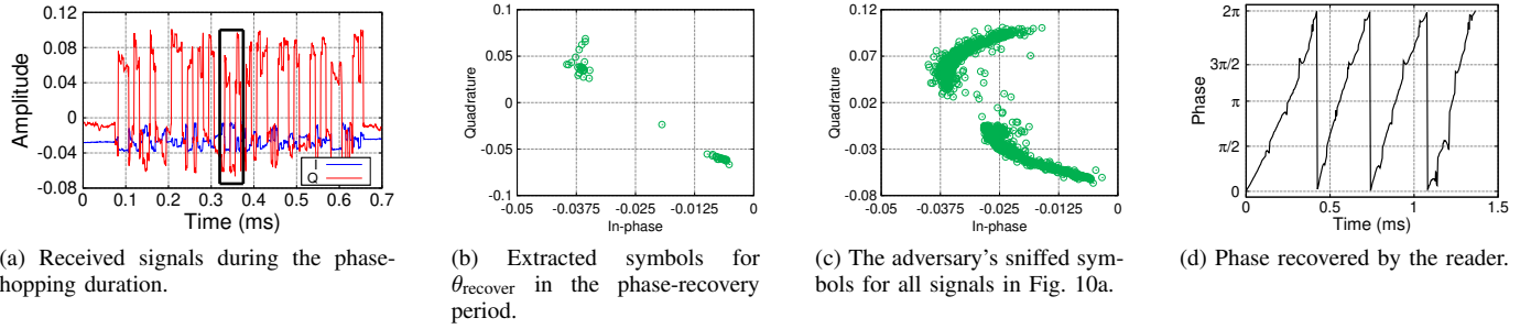
Fig. 10. Effect of reader-phase hopping.
