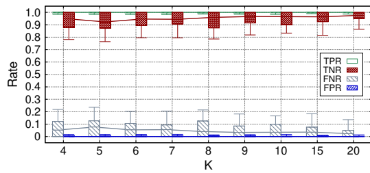
Fig. 11. Classification performance of RF-Rhythm using SVM.
